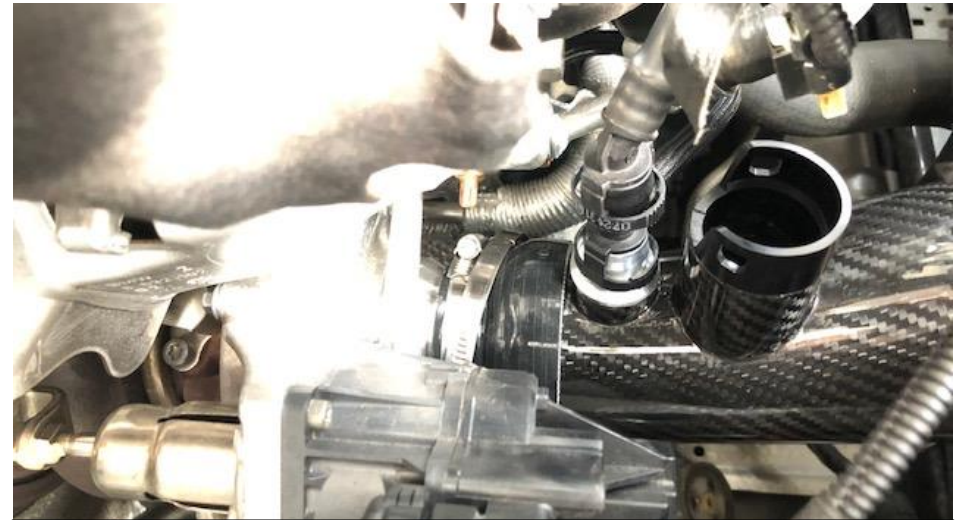
20. Insert the tube into the silicon reducer and connect the breather plug. Now secure the remaining hose clamp around the carbon tube. DO NOT OVERTIGHTEN.
